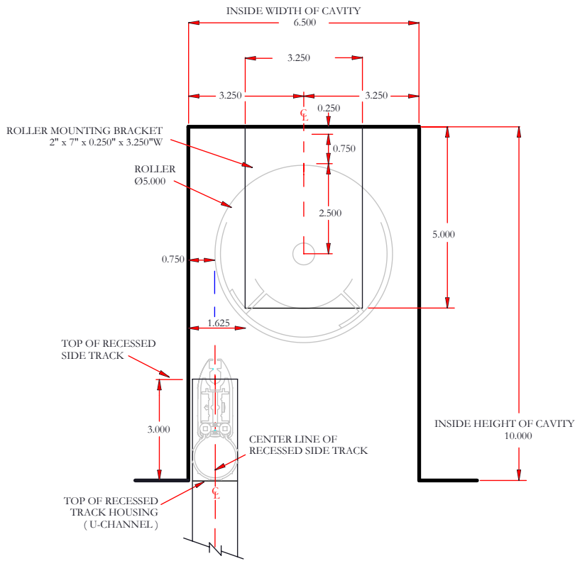
PLACEMENT OF 5" ROLLER, 5" ROLLER MOUNTING BRACKET AND RECESSED SIDE TRACK
