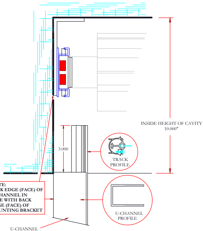
RELATIONSHIP OF THE SIDE TRACK U-CHANNEL TO THE 5" MOTOR MOUNTING BRACKET
